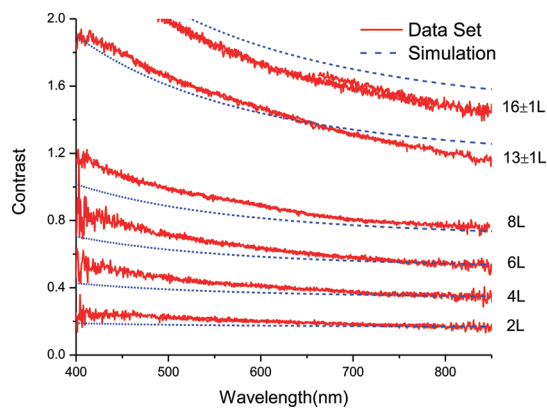
Figure 1. Simulated and experimental contrast for pristine graphene from 2 to 16 \pm 1 L.
