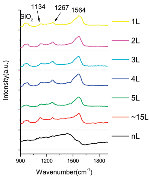
Figure 7. The Raman spectra of potassium exposed graphene as a function of L .
